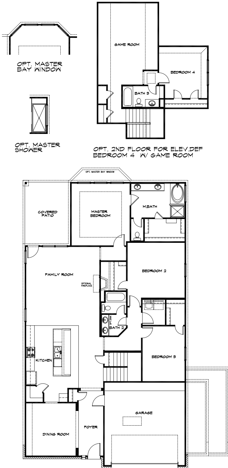
OPT. PLAN W/2ND FLOOR FOR ELE.DEF FIRST FLOOR PLAN
